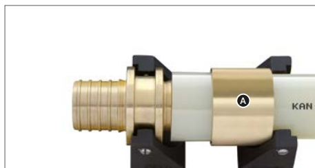
Installation of connectors (opposite side) \varnothing 12 \times 2 , \varnothing 14 \times 2 , \varnothing 18 \times 2 , \varnothing 18 \times 2,5
