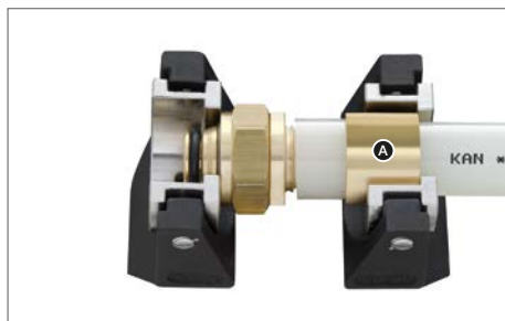
Installation of screw joint with sliding ring
